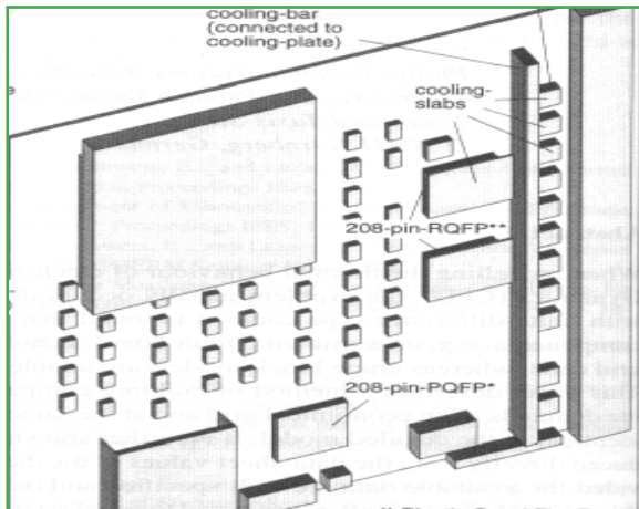
Figure 7a. Typical Telecom Cabinet. (Philips Communications Industrie AG)
